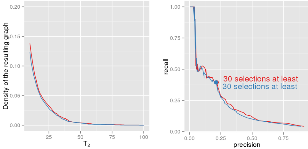
Figure 5. Evolution of the density versus T_2 for the 2 conditions (left) and Precision/Recall curve (with varying T_2 ) for the total number of edges of the true child networks compared to the corresponding inferred network. T_1 = 250 , \mu = 1 .
