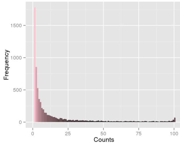
Figure 6. Distribution of the number of times an edge is selected over 100 bootstrap samples for the expression data before the diet.
