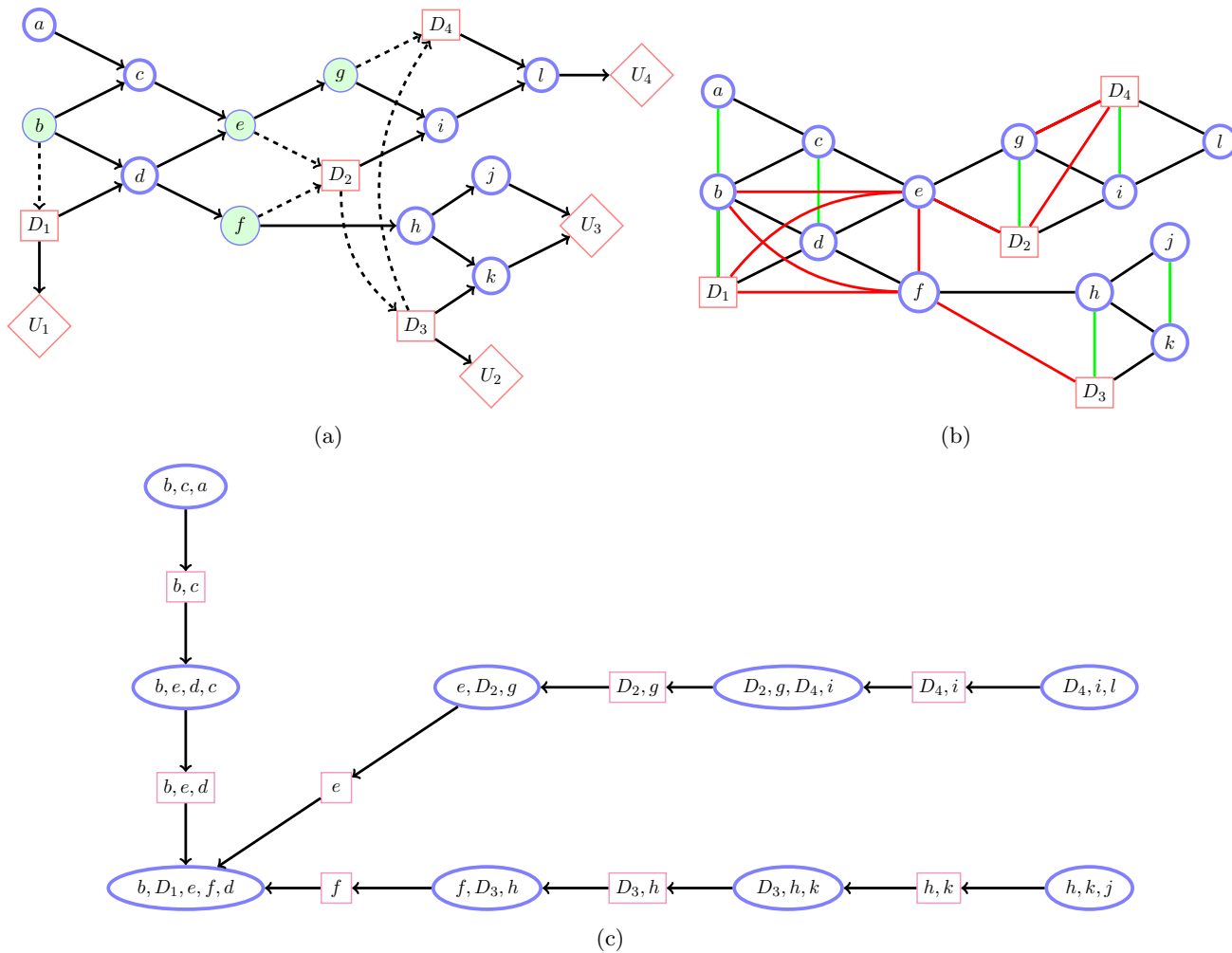
Figure 7.8: (a) : Influence Diagram, adapted from [146]. Causal consistency is satisfied since there is a directed path linking the all decisions in sequence. The partial ordering is b \prec D_1 \prec (e, f) \prec D_2 \prec (\cdot) \prec D_3 \prec g \prec D_4 \prec (a, c, d, h, i, j, k, l) . (b) : Moralised and strongly triangulated graph. Moralisation links are in green, strong triangulation links are in red. (c) : Strong Junction Tree. Absorption passes information from the leaves of the tree towards the root.
