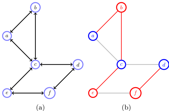
Figure 28.11: (a): A graph with bidirectional weights w_{ij} = w_{ji} . (b): A graph cut partitions the nodes into two groups \mathcal{S} (blue) and \mathcal{T} (red). The weight of the cut is the sum of the edge weights from \mathcal{S} (blue) to \mathcal{T} (red). Intuitively, it is clear that after assigning nodes to state 1 (for blue) and 0 (red) that the weight of the cut corresponds to the summed weights of neighbours in different states. Here we highlight those weight contributions. The non-highlighted edges do not contribute to the cut weight. Note that only one of the edge directions contributes to the cut.
