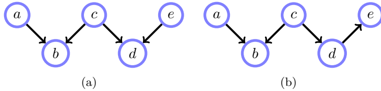
Figure 3.8: Examples for d-separation. (a): b d-separates a from e . The joint variables \{b, d\} d-connect a and e . (b): c and e are (unconditionally) d-connected. b d-connects a and e .
