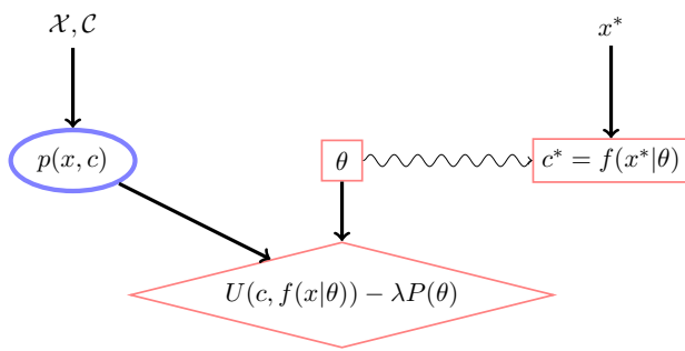
Figure 13.4: Empirical risk approach. Given the dataset \mathcal{X}, \mathcal{C} , a model of the data p(x, c) is made, usually using the empirical distribution. For a classifier f(x|\theta) , the parameter \theta is learned by maximising the penalised empirical utility (or minimising empirical risk) with respect to \theta . The penalty parameter \lambda is set by validation. A novel input x^* is then assigned to class f(x^*|\theta) , given this optimal \theta .
