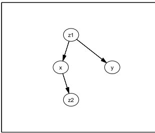
Figure 9.12: Conditional independence test of x \perp\!\!\!\perp y \mid z_1, z_2 with x, y, z_1, z_2 having 3, 2, 4, 2 states respectively. From the oracle Belief network shown, in each experiment the tables are drawn at random and 20 examples are sampled to form a dataset. For each dataset a test is carried out to determine if x and y are independent conditioned on z_1, z_2 (the correct answer being that they are independent). Over 500 experiments, the Bayesian conditional independence test correctly states that the variables are conditionally independent 74% of the time, compared with only 50% accuracy using the chi-square mutual information test. See demoCondindepEmp.m .
