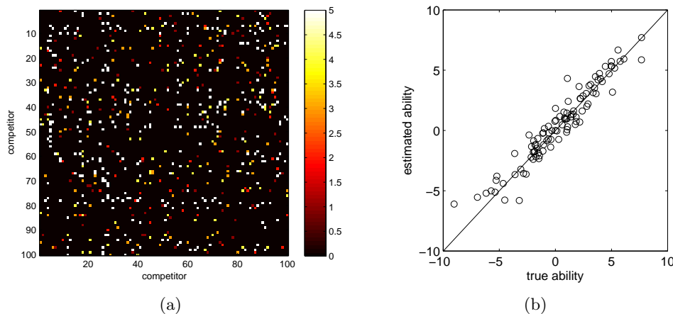
Figure 22.3: BTL model. (a) : The data \mathbf{X} with X_{ij} being the number of times that competitor i beat competitor j . (b) : The true versus estimated ability. Even though the data is quite sparse, a reasonable estimate of the latent ability of each competitor is found.
