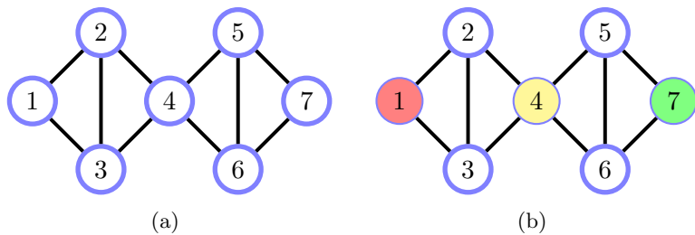
Figure 4.2: (a): \phi(1, 2, 3)\phi(2, 3, 4)\phi(4, 5, 6)\phi(5, 6, 7) . (b): By the global Markov property, since every path from 1 to 7 passes through 4, then 1 \perp\!\!\!\perp 7 \mid 4 .
