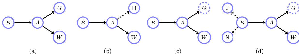
Figure 3.2: (a) : Mr Holmes’ burglary worries as given in [220]: (B)urglar, (A)larm, (W)atson, Mrs (G)ibbon. (b) : Virtual Evidence can be represented by a dashed line. (c) : Modified problem. Mrs Gibbon is not drinking but somewhat deaf; we represent such uncertain (soft-evidence) by a circle. (d) : Holmes gets additional information from his neighbour Mrs (N)osy and informant Dodgy (J)oe.
