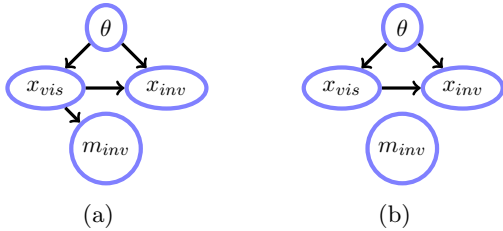
Figure 11.1: (a): Missing at random assumption. (b): Missing completely at random assumption.
