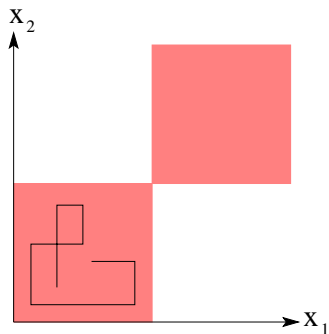
Figure 27.6: A two dimensional distribution for which Gibbs sampling fails. The distribution has mass only in the shaded quadrants. Gibbs sampling proceeds from the l^{\text{th}} sample state (x_1^l, x_2^l) and then sampling from p(x_2|x_1^l) , which we write (x_1^{l+1}, x_2^{l+1}) where x_1^{l+1} = x_1^l . One then continues with a sample from p(x_1|x_2 = x_2^{l+1}) , etc. If we start in the lower left quadrant and proceed this way, the upper right region is never explored.
