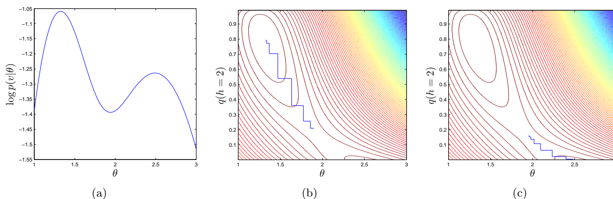
Figure 11.2: (a) : The log likelihood for the model described in example(51). (b) : Contours of the lower bound LB(q(h=2), \theta) . For an initial choice q(h=2) = 0.5 and \theta = 1.9 , successive updates of the E (vertical) and M (horizontal) steps are plotted. (c) : Starting at \theta = 1.95 , the EM algorithm converges to a local optimum.
