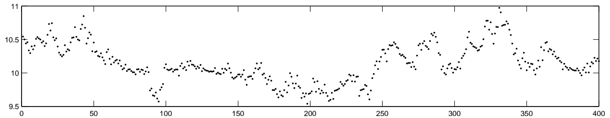
Figure 25.11: Data from an intermittent mean-reverting process. See exercise(242).
