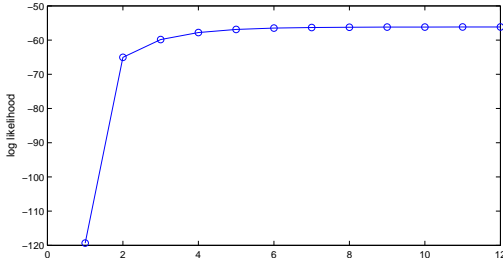
Figure 11.4: Evolution of the log-likelihood versus iterations under the EM training procedure (from solving the Printer Nightmare with missing data, exercise(139)). Note how rapid progress is made at the beginning, but convergence can be slow.
