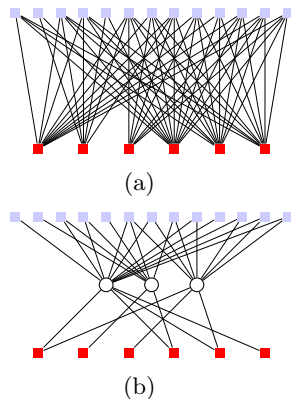
Figure 20.17: Graphical representation of dyadic data. (a) : There are 6 documents and 13 words. A link represents that a particular word-document pair occurs in the dataset. (b) : A latent decomposition of (a) using 3 ‘topics’. A topic corresponds to a collection of words, and each document a collection of topics. The open nodes indicate latent variables.
