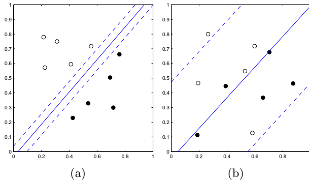
Figure 17.12: The decision boundary p(c = 1|\mathbf{x}) = 0.5 (solid line) and confidence boundaries p(c = 1|\mathbf{x}) = 0.9 and p(c = 1|\mathbf{x}) = 0.1 and 10000 iterations of batch gradient ascent with \eta = 0.1 . (a): Linearly separable data. (b): Non-linearly separable data. Note how the confidence interval remains broad, see demoLogReg.m .
